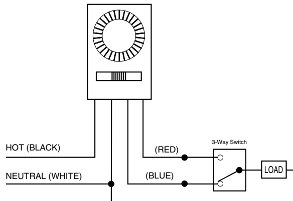
3-Way Installation
